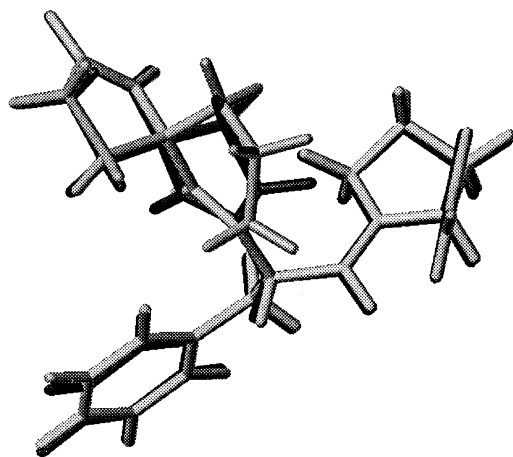
Figure 2. Compound 6 =black; Compound 8 =grey.
